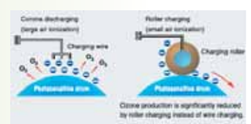
Corona Discharging and Roller Charging
